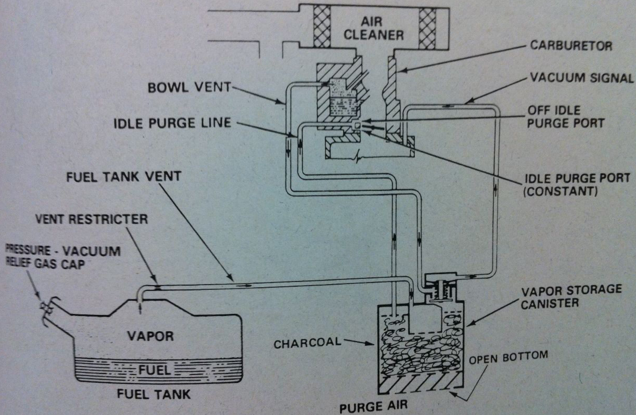
10.2 Typical late model EECS system component layout
